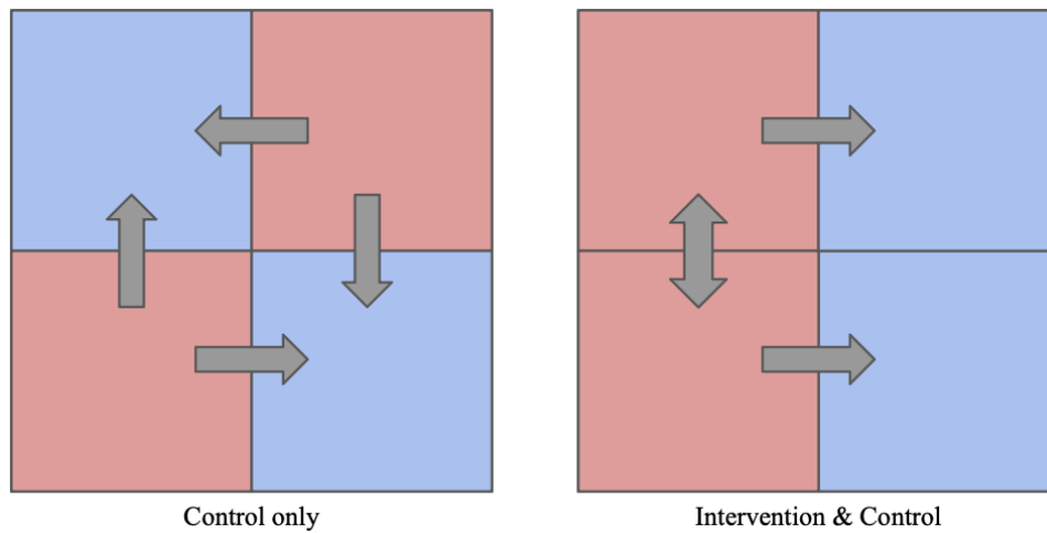
Figure 4: (Left) Spillover application from intervention cells (red) to only control cells (blue) & (Right) spillover application to intervention (red) and control cells (blue).
